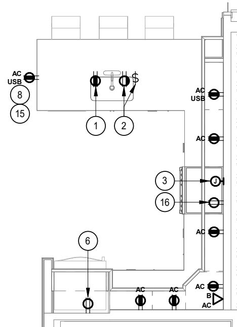
2 E501 ENLARGED 'BLUEBIRD' UNIT KITCHEN POWER PLAN SCALE: 1/4" = 1'-0"
