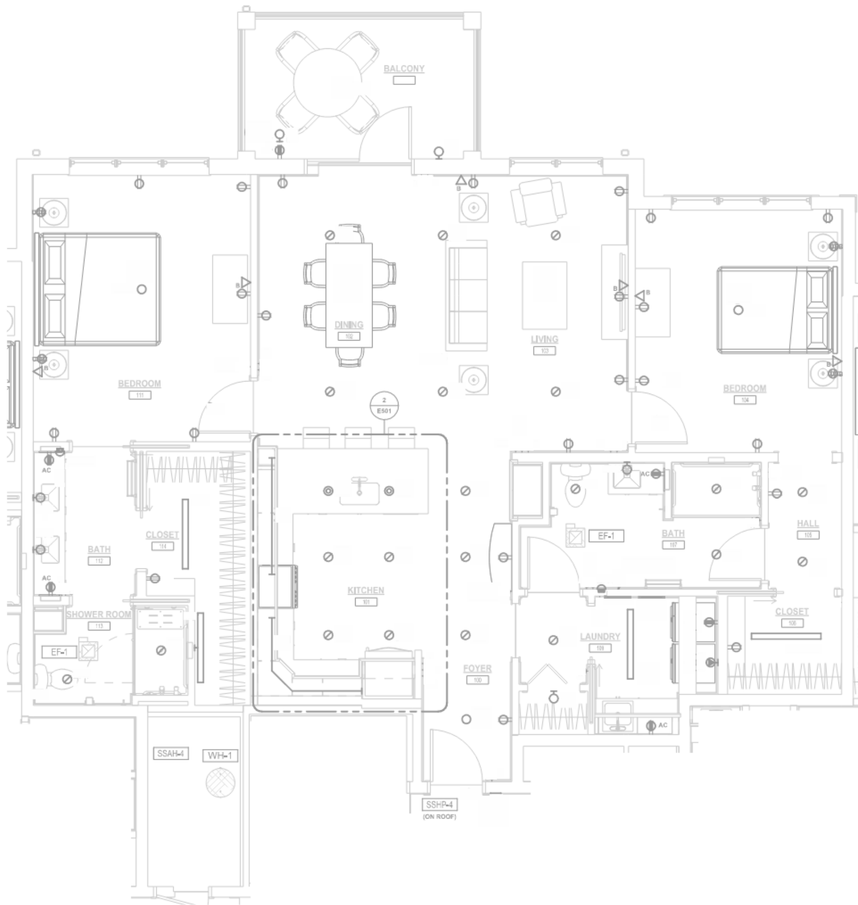
1 E501 ENLARGED 'BLUEBIRD' UNIT ELECTRICAL PLAN SCALE: 1/4" = 1'-0"
